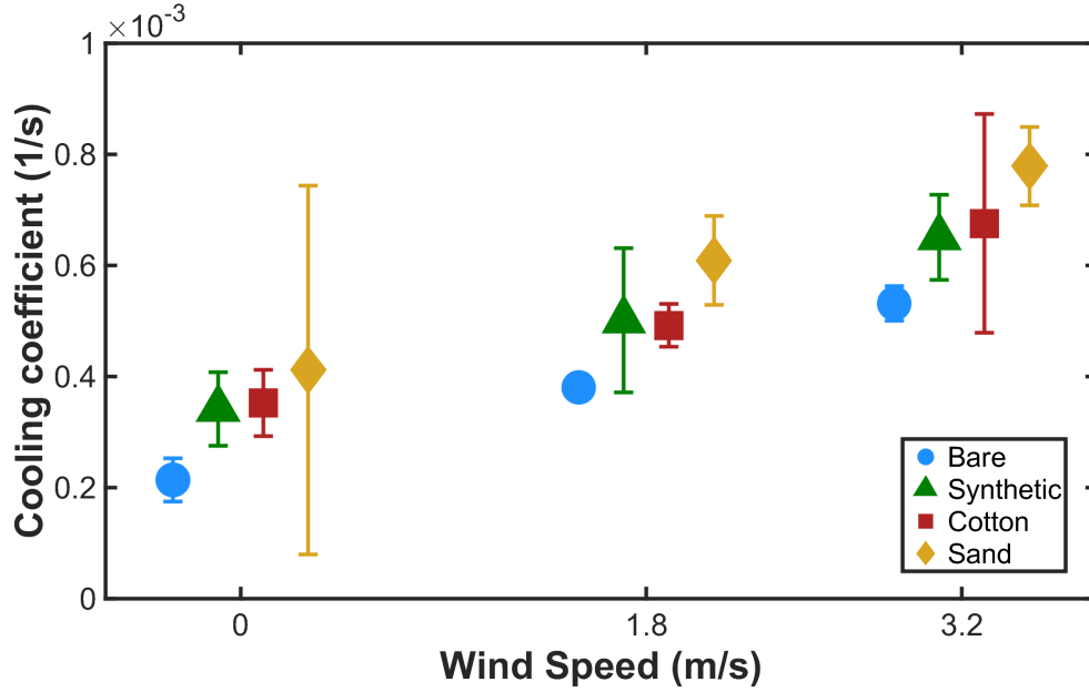
Fig. 10: Cooling coefficients plotted as a function of wind speed and the markers organized by material type. The data points are staggered at each wind speed to improve readability.
