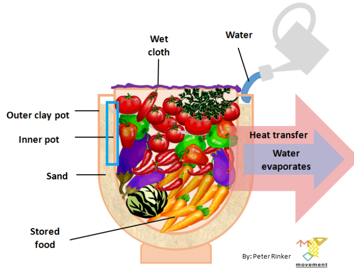
Fig. 3: Cartoon cross section of a pot-in-pot refrigerator [6]. Water is poured into the sand between the two pots and evaporates through the outer pot, cooling the food in the inner pot. The blue box marks the portion of the device analogous to the experimental setup.
