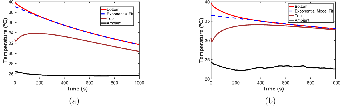
Fig. 9: (a) Sand with wind speed of 3.2 m/s. (b) Sand with wind speed of 0 m/s. Notice the difference in the fit curve towards the beginning of the data collection period.
