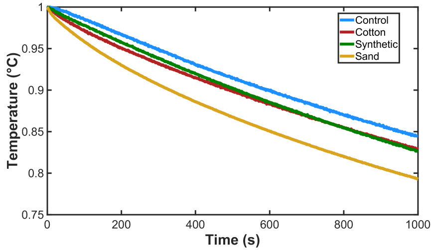
Fig. 8: Ratio of temperature at time t to initial temperature over the data collection period. Note the improved cooling by placing a wet material on the block.
