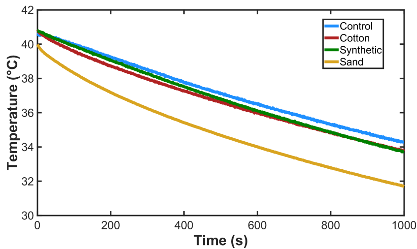
Fig. 7: Temperature at the bottom surface of the block as a function of time with wind speed of 3.2 m/s. Note the initial temperatures are different, so direct comparisons are difficult to make from this graph.
