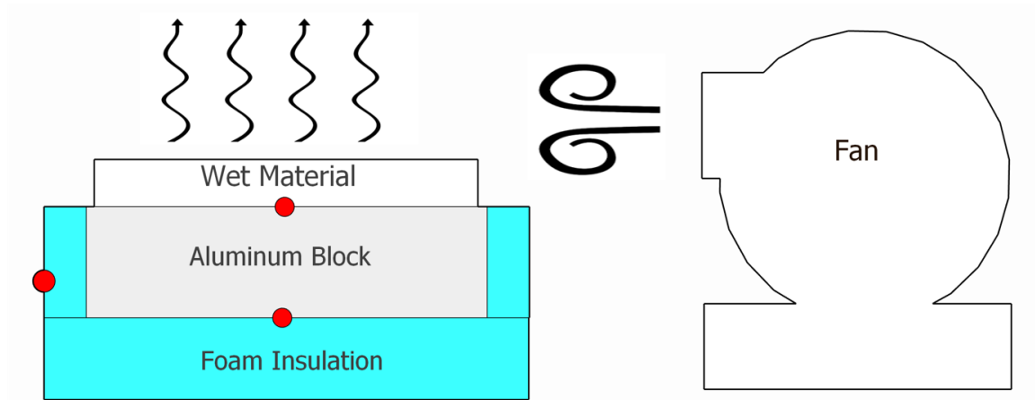
Fig. 6: Schematic of experimental setup with a fan blowing over the water-soaked material. Temperature sensors (red dots) are placed to record the temperature at the top and bottom of the block and the ambient air. These are connected to Logger Pro data collection units (not pictured).
